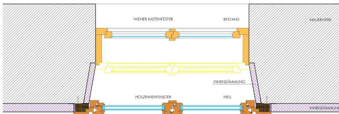
Kaiser Street: Box-type window with interior insulation, old interior wing shown in yellow (Source: AKP)
